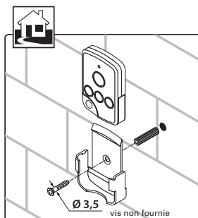
Fixation murale
