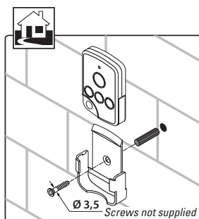
Wall attachment Ø 3,5 Screws not supplied
